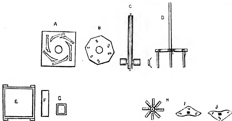
479— Gatiss' Central Discharge Water Wheel.
