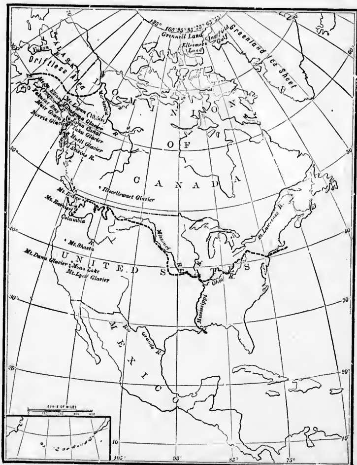
Sketch map showing the distribution of some of the better-known glaciers of North America. Southern limit of Pleistocene ice sheet indicated by a heavy broken line.
