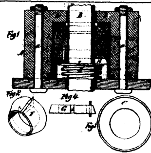
6233 Wright and Schueble's Improvements in Piston Packings.
