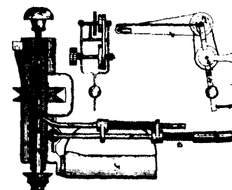
6243 Dodge and Fifield's Improvements on Machines for Burnishing the Edges of Shoe Soles.
