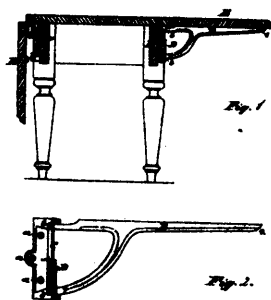
4533 McElroy's Table-leaf Support.
