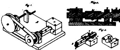
4527 Toppan, Meloon, Chapin &amp; Meloon's Wood Planing Machine.
