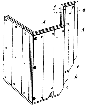
36887 Wakefield's Sheet Piling for Dams, &amp;c.
