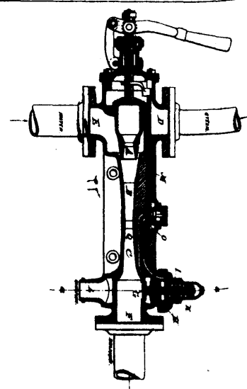
18354 Schatte's Steam Injector.
