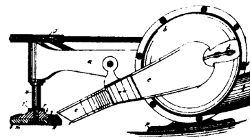
14055 Stevens's Improvements on Buffing Machines for the Soles of Boots and Shoes.
