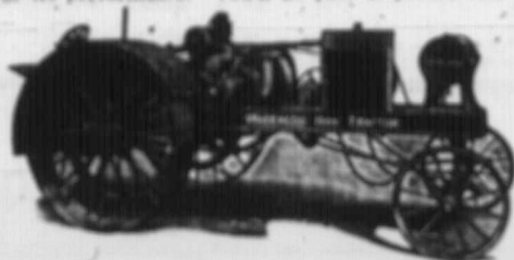
Weight only 600 lbs. Brake Test 24 h.p. | Draw Bar 12 h.p. | 12 gears, High Traction Drive Magnets, 100% Ignition Starter
