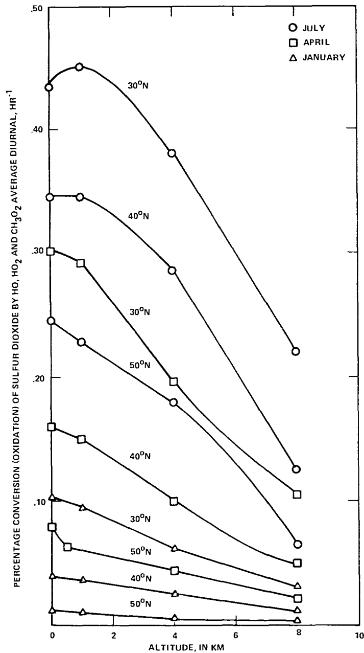
Figure 4.4 Daily average S 2 O oxidation as a function of altitude for various latitudes and months. (from Altshuller, 1979)
