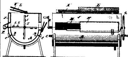
14119 Dufort & Eldridge's Improvements on Feather Renovators.
