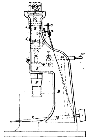
32589 Glossop's Pneumatic Hammer.
