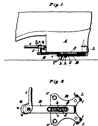
32592 Coe's Ice Creeper.
