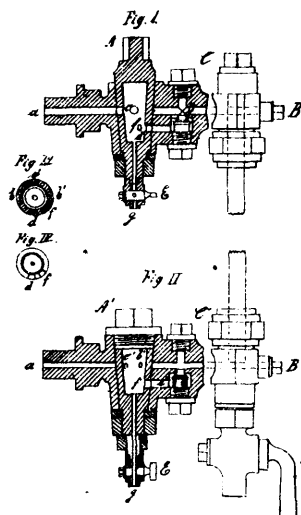
32595 Svensson's Water Gauge Cock.
