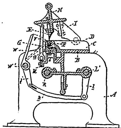
30019 Ward's Hoop Cutting Machine.
