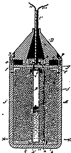
30017 Vigil and Revueltas' Shoal Water Indicator.
