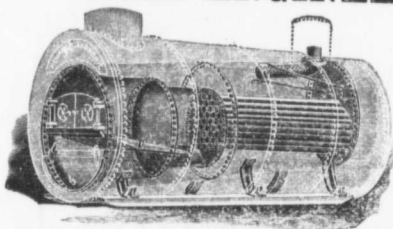
THE MONARCH ECONOMIC BOILER.
