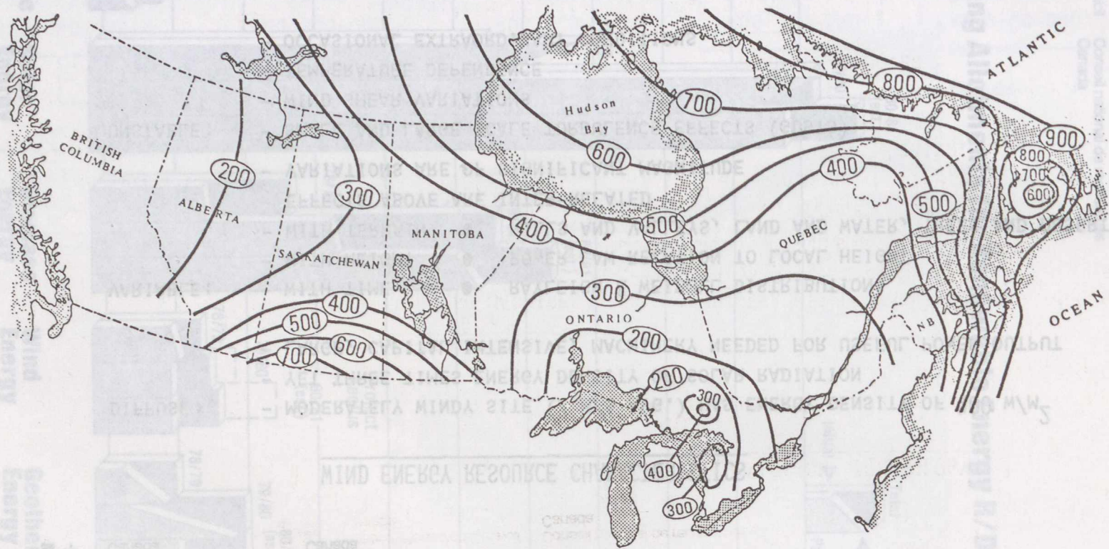
ANNUAL AVERAGE WIND ENERGY DENSITY AT 50m ALTITUDE
