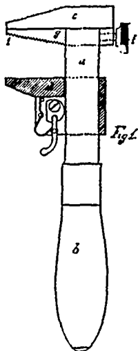
28724 Atwater's Removable Jaw for Wrenches.
