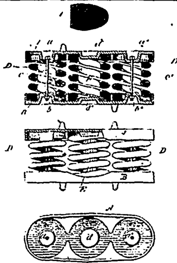
22990 Coghlin's Spring for Railway Cars.
