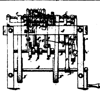
3460 Smith's Machine for Making Clothes Pins.
