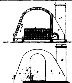
3450 Williams & Edwards' Improvements in Kilsns for Burning or Drying Bricks, Tiles and Earthenware and Mode of Setting the Material to be Burned or Dried.
