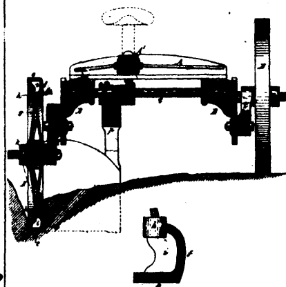
18129 Wiard's Improvements in Sulky Ploughs.
