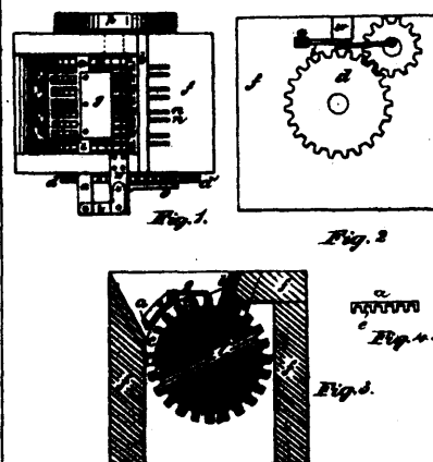
18126 Phelps' Grain Cutting Machine.
