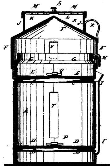
18128 Johnson's Improvements in Cooking Steamers.
