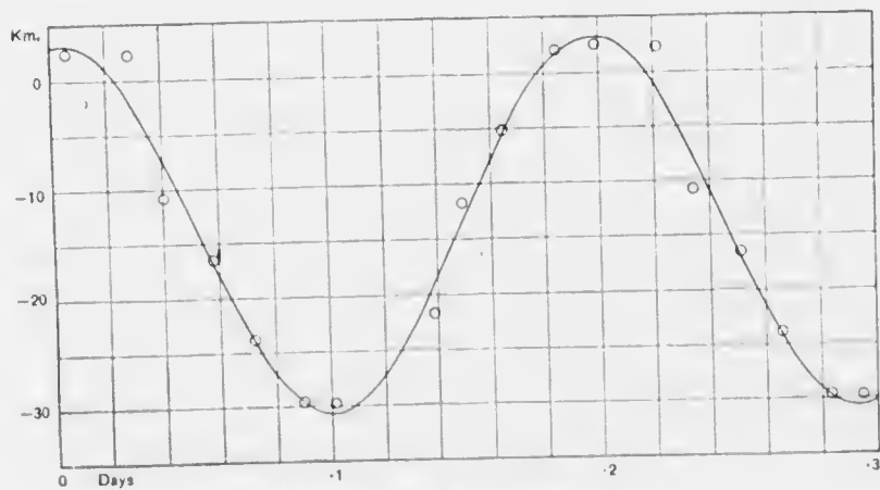
VELOCITY CURVE OF 12 LACERTE.
