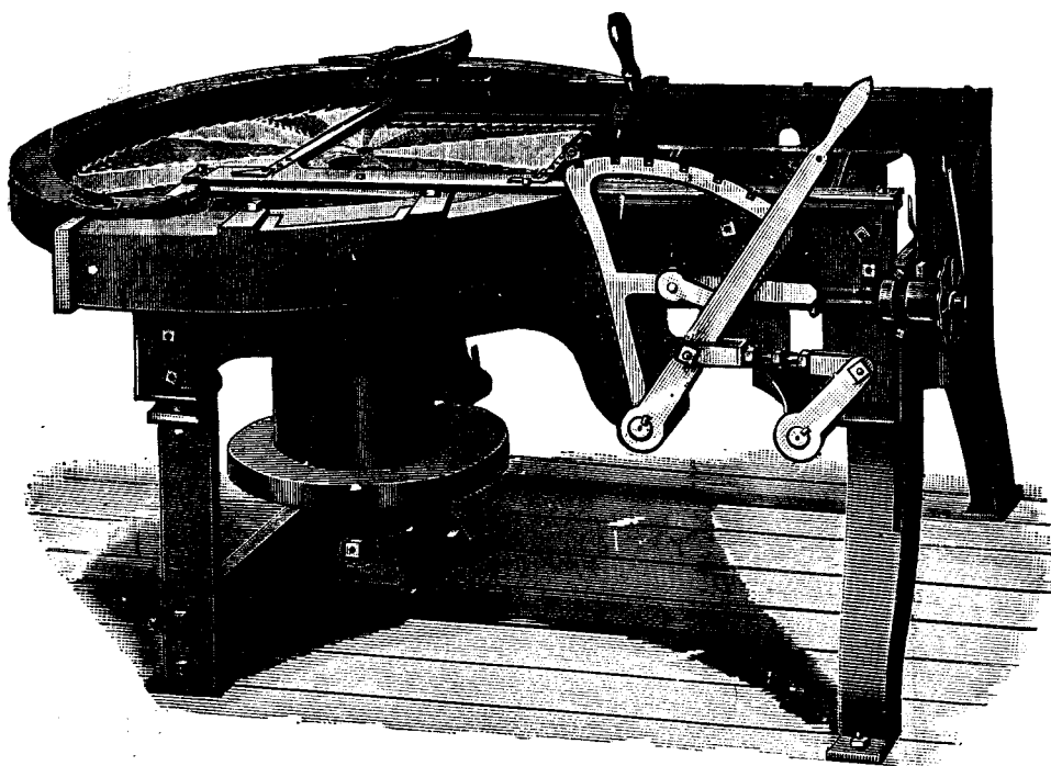
DAUNTLESS SHINGLE AND HEADING MACHINE. Takes Saws up to 42" diameter. Capacity 25,000 to 50,000 per day.
