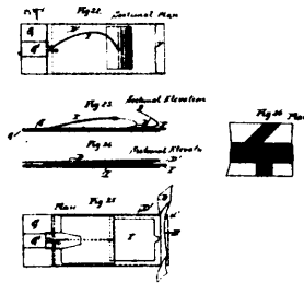
8519 Fole's Improvements on Ticket Registers.
