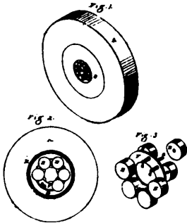
8512 King's Antifriction Bearing for Shafts and Axes.
