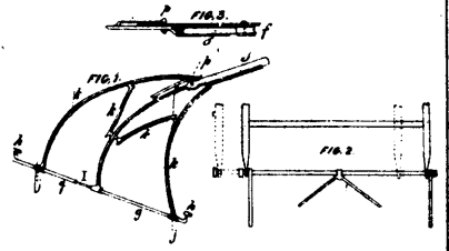
8514 Cleveland's Adjustment of Carriage-Poles and Shafts.
