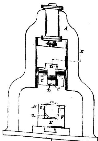
Facer's Steam Hammer.
