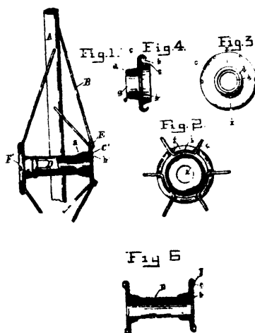
Gendron's Vehicle Wheel.
