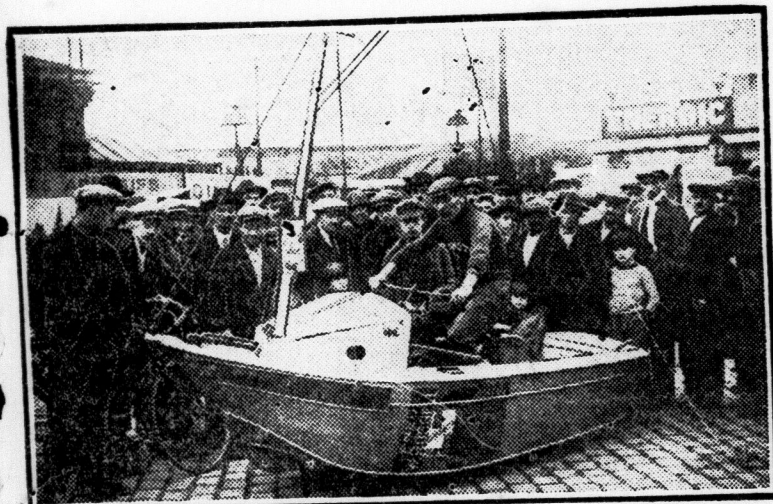
Marius Gallee of Paris, with the novel amphibian boat in which he travelled from Paris to Amsterdam, Holland. He built it around a bicycle.
