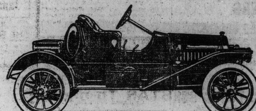
Model "25" Roadster, $1,450, Fully Equipped. Motor, 3½x4½. 105-inch wheel base. Tires, 32x3½. Trunk, $15 extra. Gasoline tank in rear.
