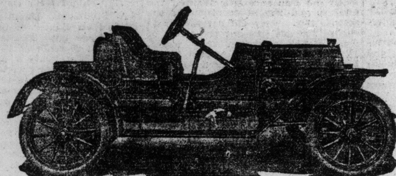
Model "22" Roadster Type, $800. Motor 5x4, water cooled. Wheel base, 96 inches. Tread, 56 inches. Tires, 30x3½. Quick detachable gasoline tank on rear.
