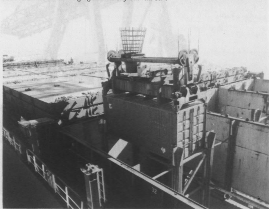
Container crane loading container into cellular containership.
