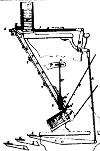
5968 Lorenz's Type Setting Machine.
