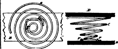
2187 Wells' Spring Bottoms for Bedsteads and Seats.
