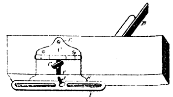
11537 Kinney's Improvements on Plane Bevelling Gauges.
