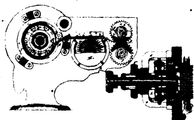
13072 Edge's Improvements on Machines for Making Wire Tubes.
