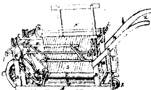
13064 Eadie's Improvements on Machines for Killing Potato Bugs.
