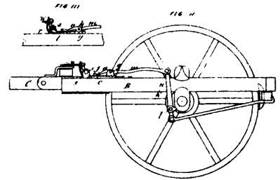
2361 Fisk's Self-Acting Waggon Brake.
