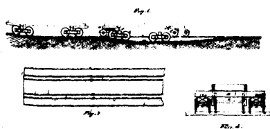
5784 Ramsay's Car Truck Shifting Apparatus.
