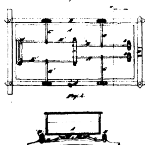
5789 Whitney's Vehicle Spring.
