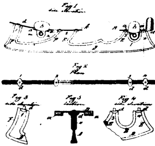
12310 Barney's Improvements in Skates.
