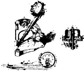
12313 Platt &amp; Bradley's Improvements on Rivet or Eyelet Setting Machines.
