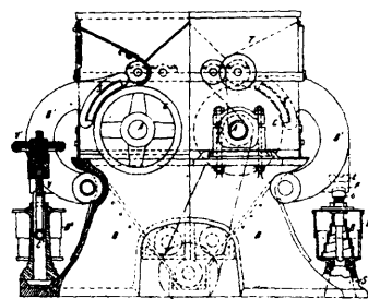
39576 Quenehen and Vansteenkiste's Machinery for Decorticating and Disintegrating Grain.
