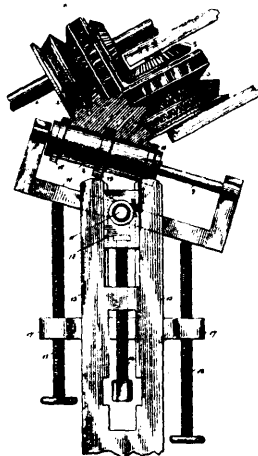
39578 Weles and Gassen's Apparatus for Producing Plastic Ornaments on Profiled Borders, etc.
