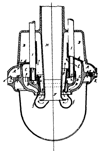
39573 Stellwag's Gas Lamp.
