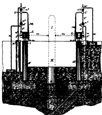
39574 Hagerty's Water Motor.
