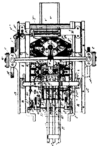
39575 Stebbins and McDonald's Machine for Making Envelopes and Placing Inclosures.
