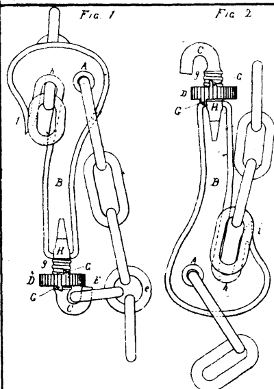
38022 Boiteau and Fortier's Grab Hook.
