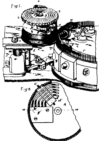
38023 Wiggin's Presser Wheel for Knitting Machines.
