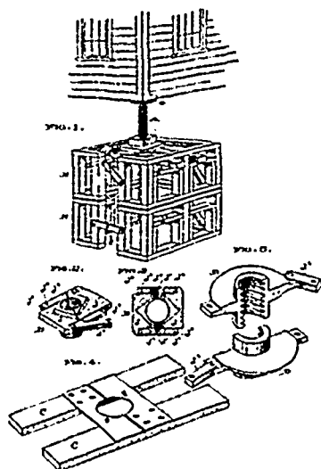
24845 Maher's House Raising Apparatus.
