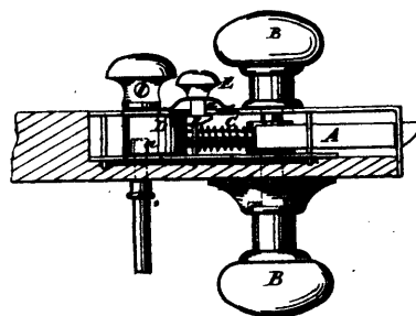
5029 Rogers' Improvements on Locks.
