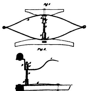
5033 Hopson & Lambie's Improvements on Vehicle Springs.
