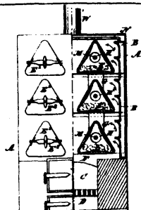
5038 Rigby's Apparatus for the Manufacture of Gas from Petroleum, &c.
