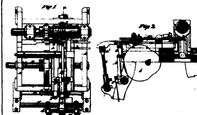
5036 Dodge's Feeding Device of Machines for Forging Nails and Spikes.
