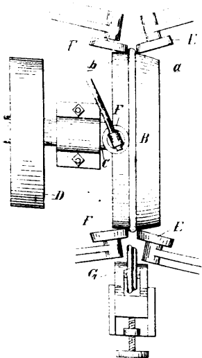
35464 Gendron's Process of Making Tires.
