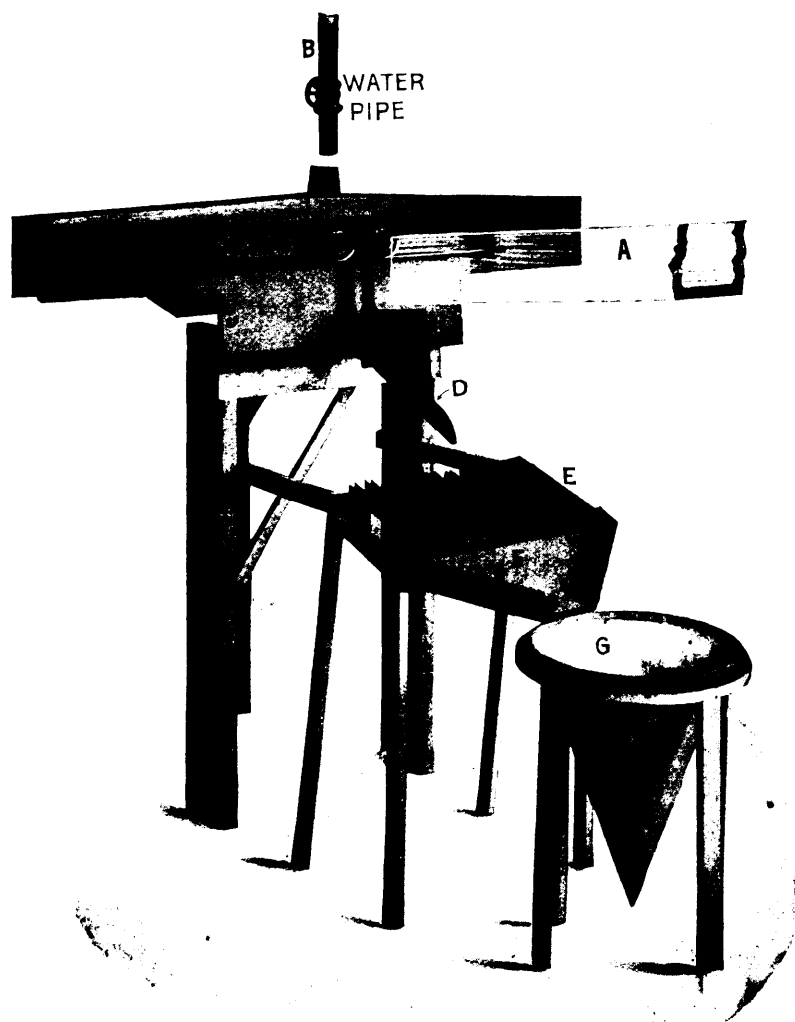
The Lamb Automatic Tailings Sampler
