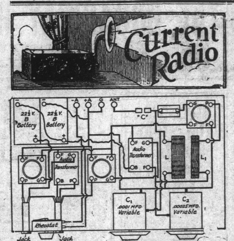
Navy Test Receiver Redesigned for Broadcast Work
