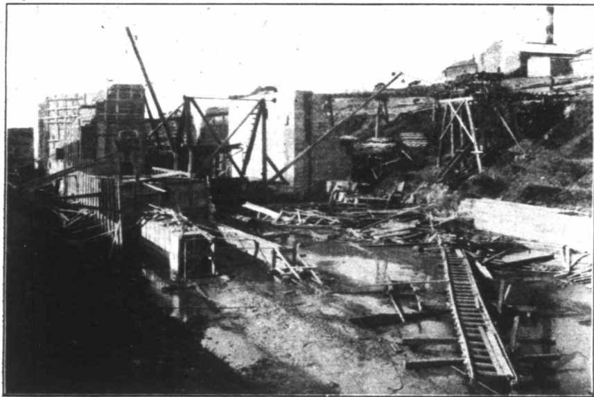
Construction of Locks, St. Andrews Rapids, Red River.
