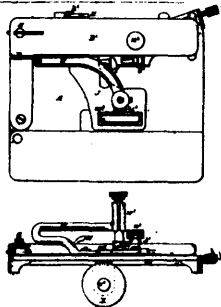
7631 Randel, Clipperly, Cole & Haslehurst's Improvements on Sewing Machines.
