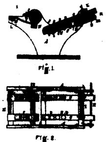
7641 Rico's Inking Apparatus for Printing Presses.
