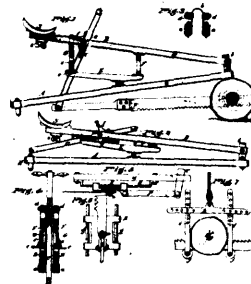
11040 Brewer's Improvements on Sawing Machines.
