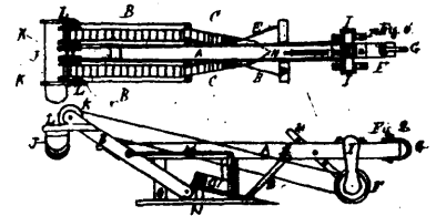
11035 Peck's Improvements on Ditching Machines.
