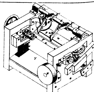
10076 Naylor's Improvements on Strip-Cutting Machines.
