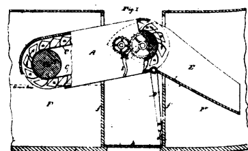
10070 Hough's Machine for Transferring Grain.
