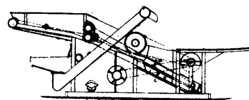
10064 Bassett's Improvements in Threshing Machines.
