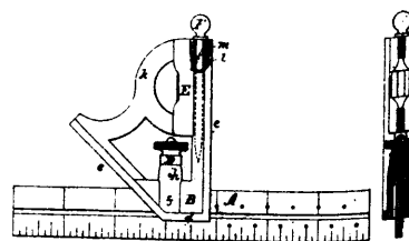
10073 Starrett's Improvement in Try Squares.
