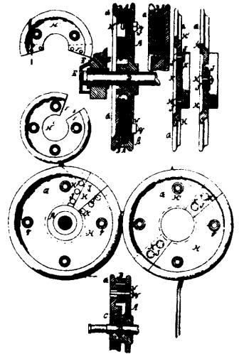
27418 Palmer's Railway Car Wheel.
