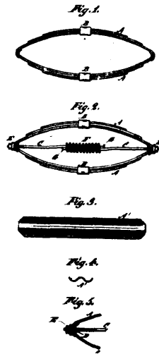
27417 Chase's Elliptic Spring.
