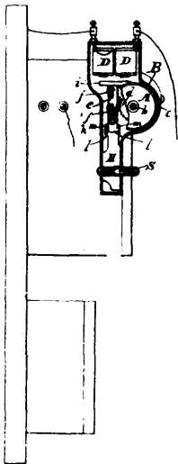
27419 Wittenberg's Telephone Register.
