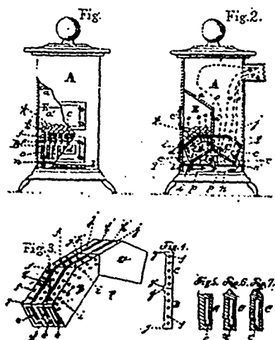
25387 Weston's Fuel Support for Stoves, etc.
