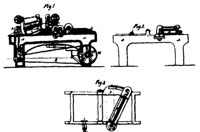
6610 Hewes, Norris, Hall and Sheldon's Door Planing Machine.
