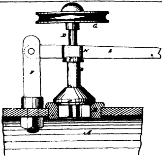
6601 Thomson's Improvement on Safety-Valves.
