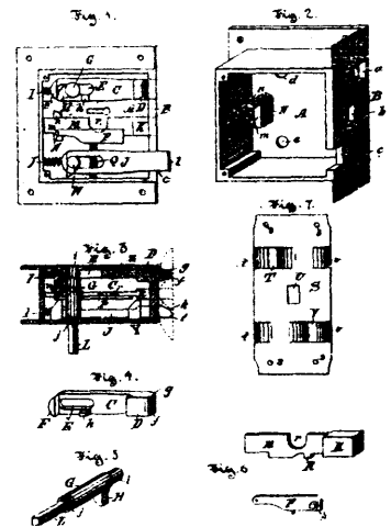
33244 Mencon's Latch and Lock.
