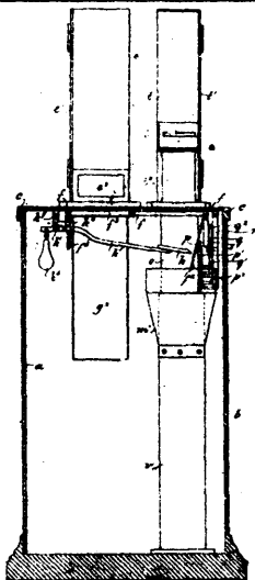
33245 Clifford's Apparatus for Receiving Coin, etc.
