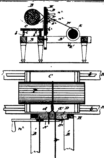
18730 Mereweather's Machine for Tying Packages with Wire.
