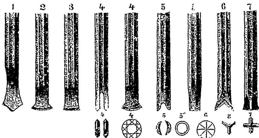
DIFFERENT FORMS OF DRILL POINTS.
